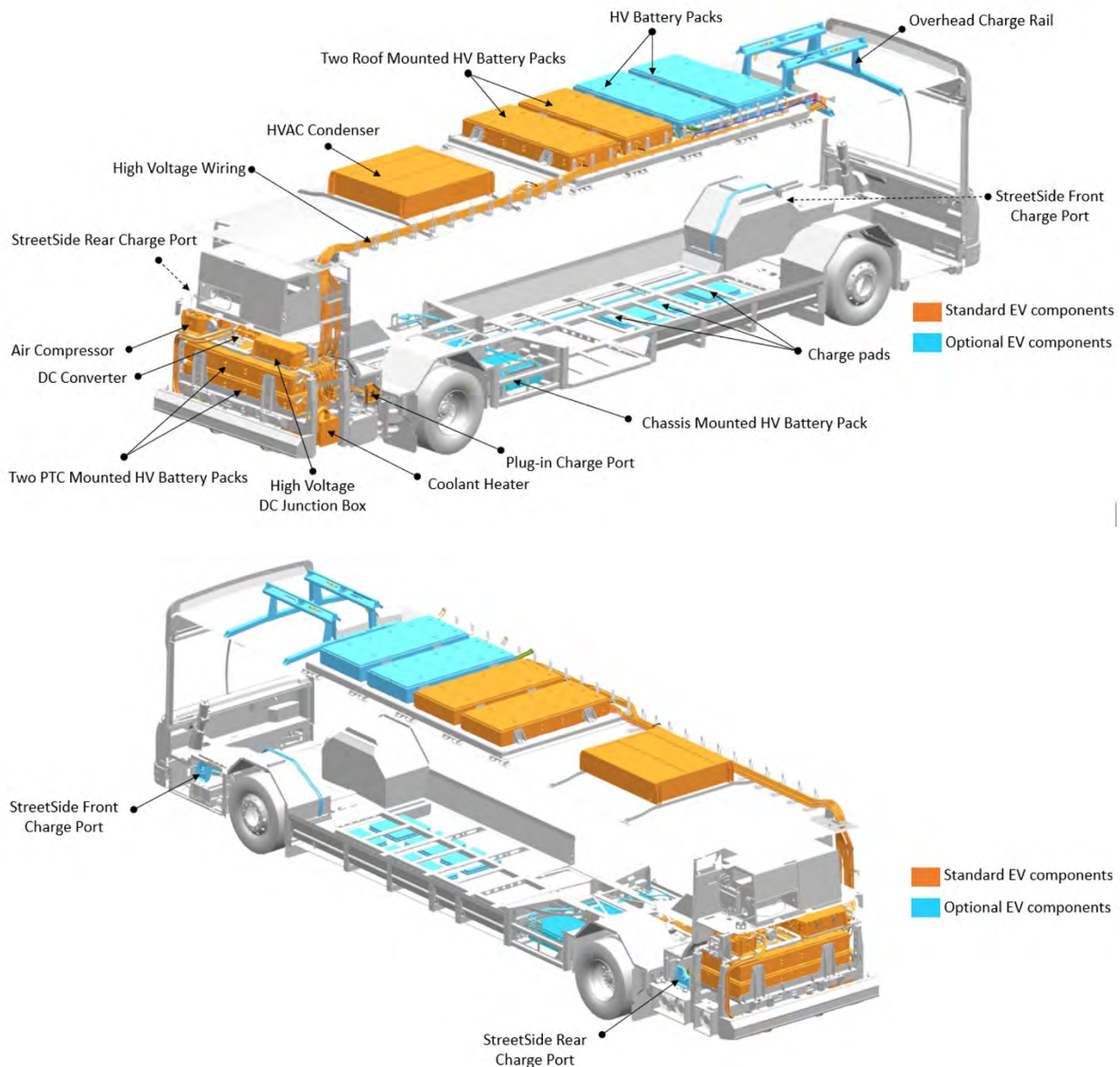
Fig. 1.8. GILLIG Battery Electric Bus High Voltage System Layout
